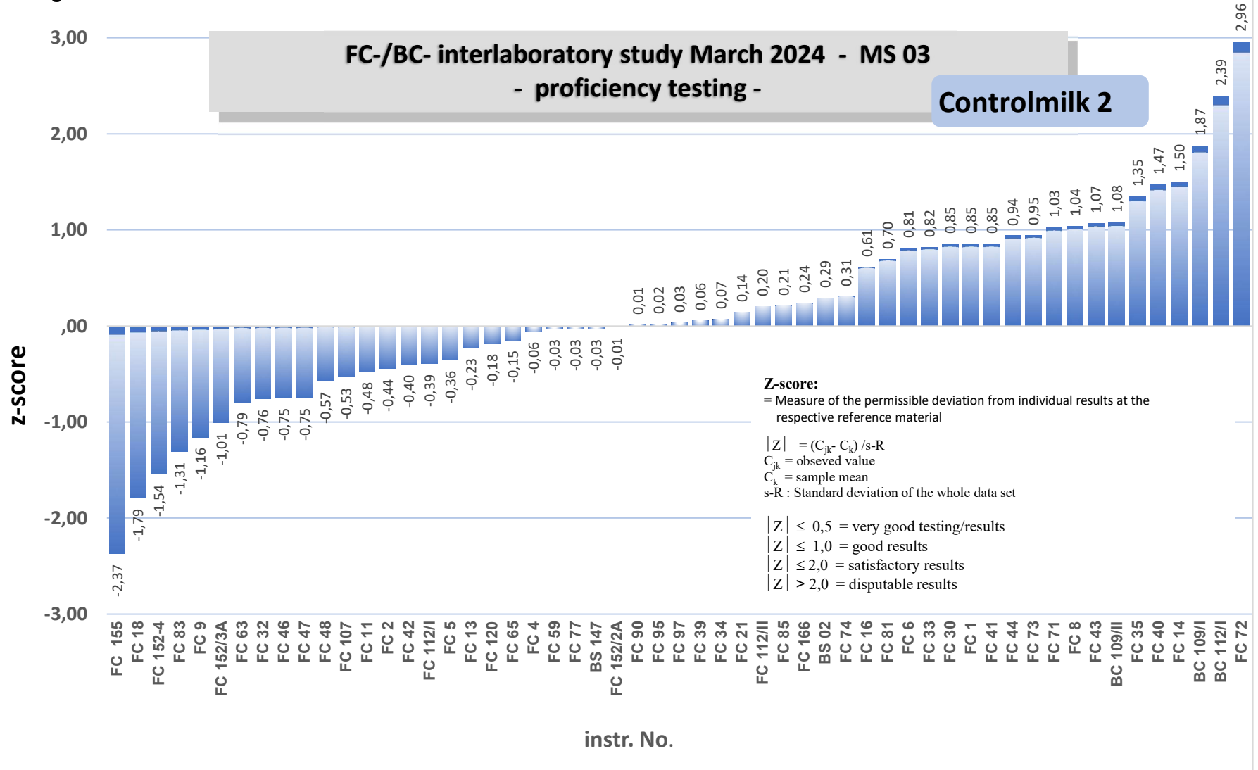
Fig.1: Difference - z-score to the mean values of Controlmilk
